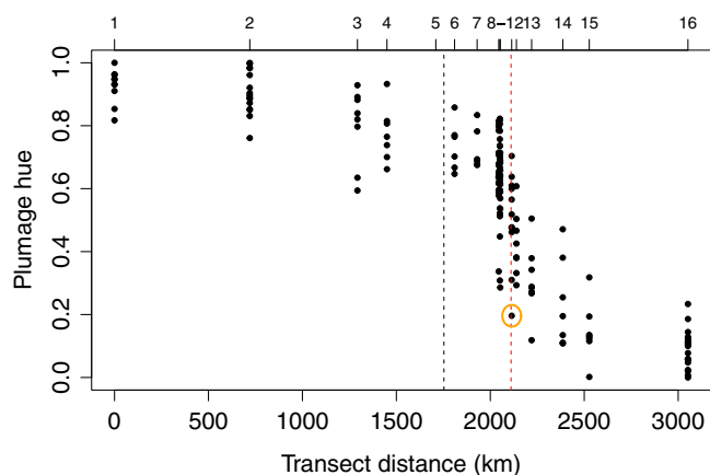
Figure 6. Variation in plumage hue across the transect, with the hybrid index (black) and plumage line (red) centers marked with dashed lines. Higher values for hue correspond to redder plumage color. At sampling location 11, at the center of the plumage line, the frequency of orange birds is 1/11 = 0.09 (represented by the circled point). Eight unlinked loci would be required for genetic dominance of red plumage alleles to explain this phenotypic frequency (see text for details). Numbers along the top refer to sampling locations.
