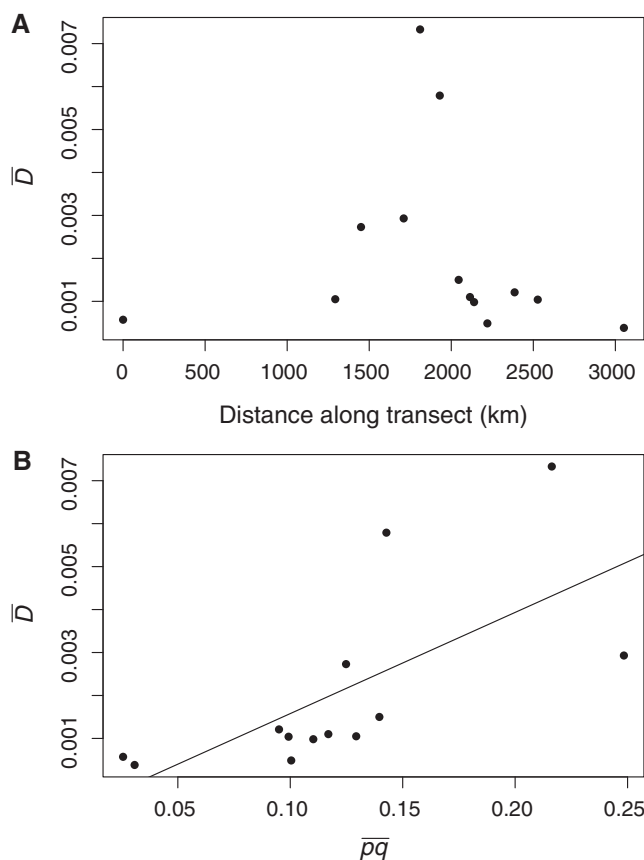
Figure 4. Average linkage disequilibrium across the 102 diagnostic loci plotted against transect distance (A) and average allele frequencies (B).
