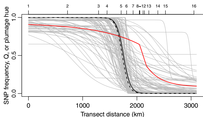
Figure 3. Combined maximum likelihood geographic clines for the 2702 loci hybrid index (HI, black), the 102 diagnostic loci hybrid index (HI diag , black dashed), each of the 102 diagnostic SNP loci (gray), and plumage hue (red). Higher values for hue correspond to redder plumage color. All SNP loci have allele frequency >0.8 on one end of the cline and <0.2 on the other end, even those with very wide-fitted clines that appear to deviate from this criterion. Numbers along the top refer to sampling locations.
